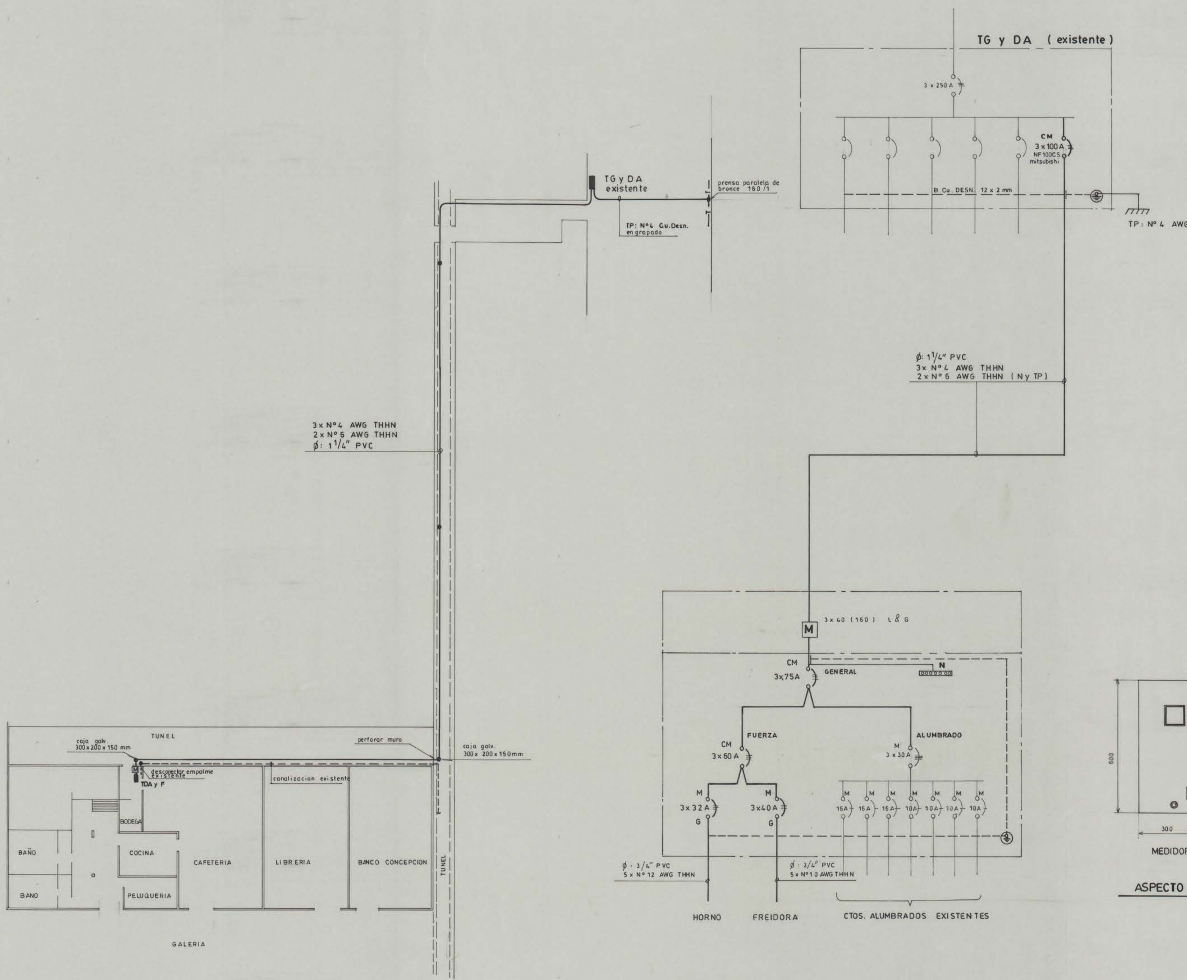
DIAGRAMA UNILINEAL
